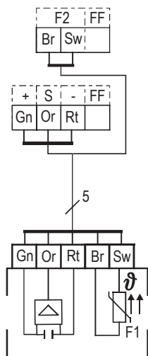
Humidity temperature sensor - FTS2:
