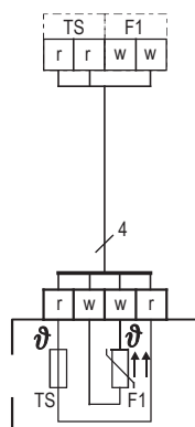
Heater sensor - F1:
